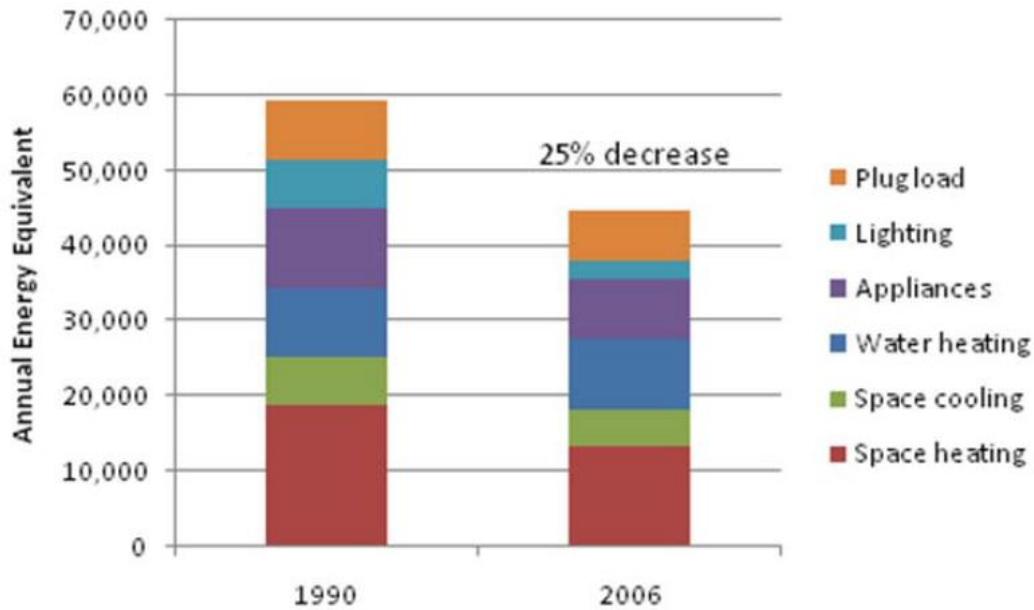
Figure 10 – Whole house energy comparison between 1990 and 2006 models – Appendix Table 8
